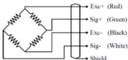
Wiring Diagram
